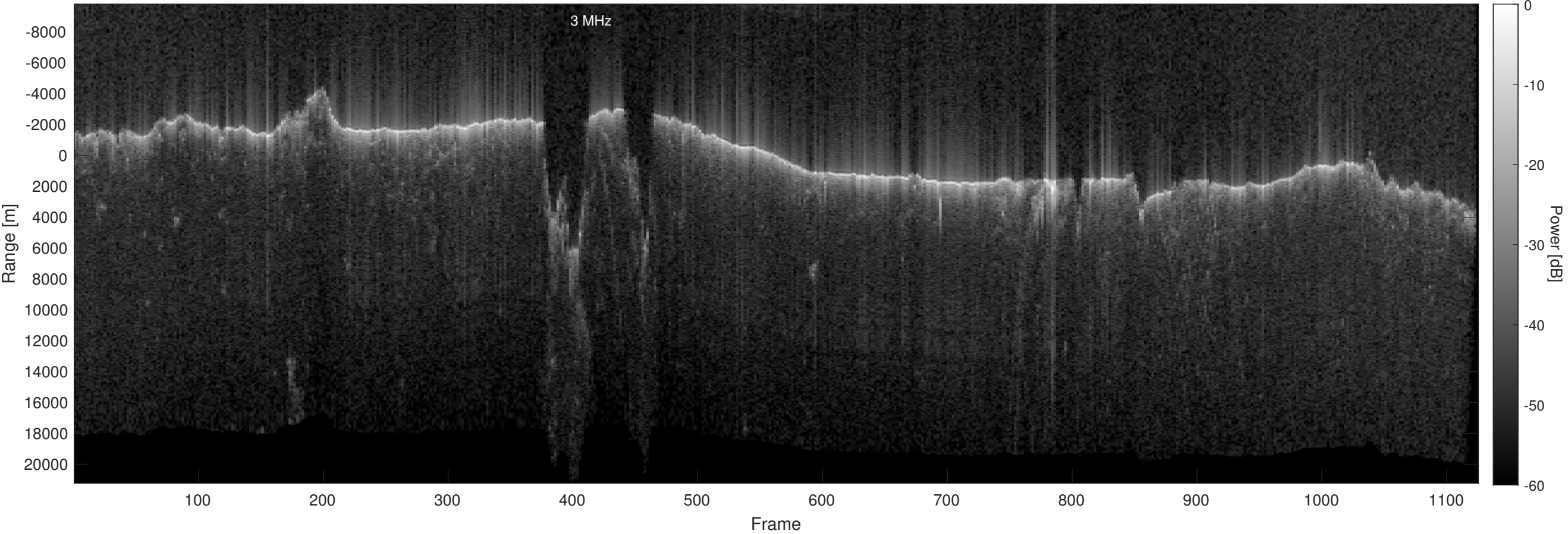
Orbit 22869, Optimized, No Window, Depth-Corrected, Channel 2
