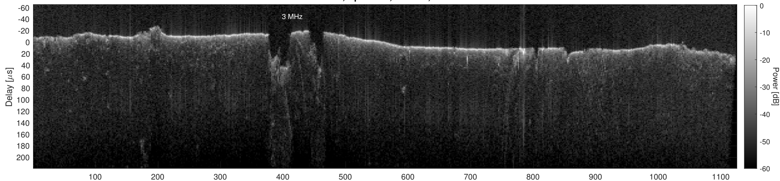
Orbit 22869, Cluttergram
