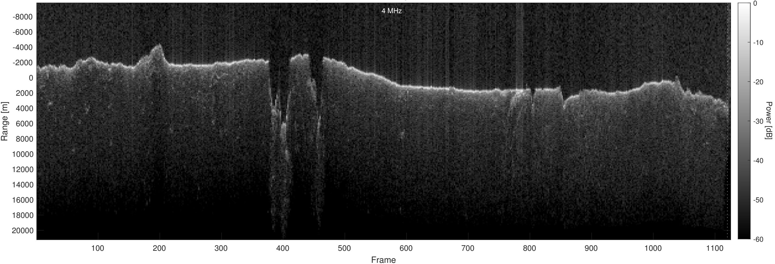
Orbit 22869, Optimized, Window, Depth-Corrected, Channel 2
