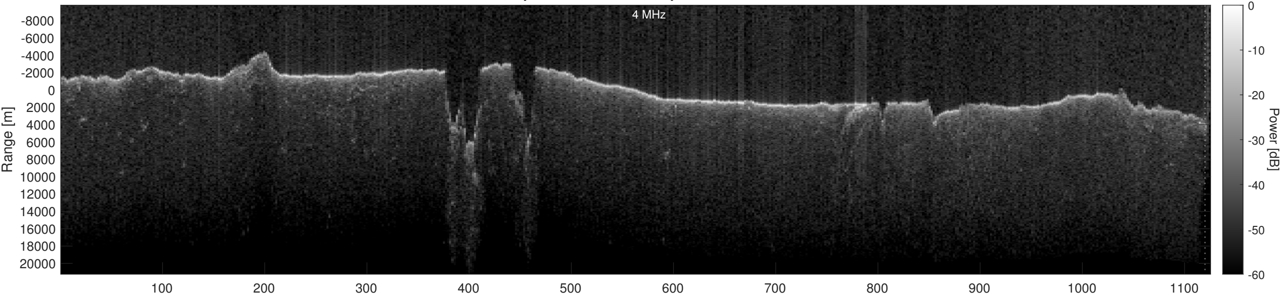
Orbit 22869, Optimized, Window, Depth-Corrected, Channel 2
