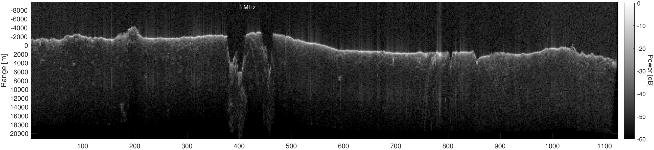
Orbit 22869, Depth-Corrected Cluttergram
