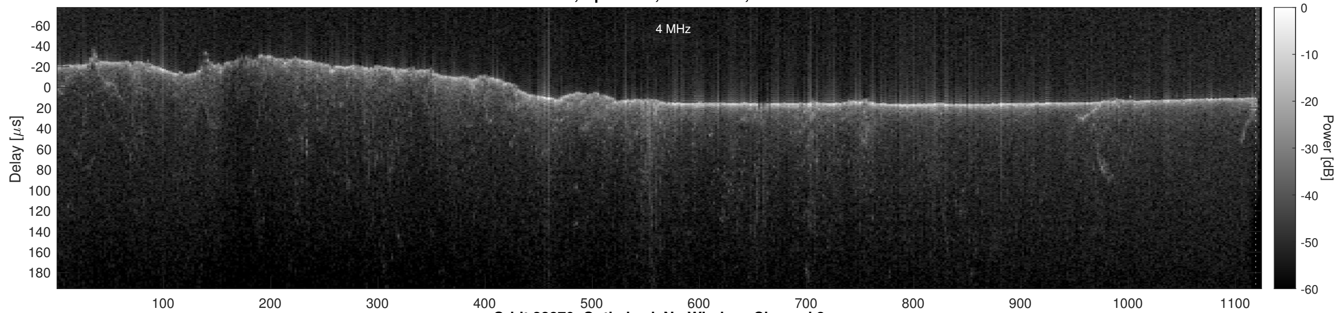
Orbit 22870, Optimized, No Window, Channel 2
