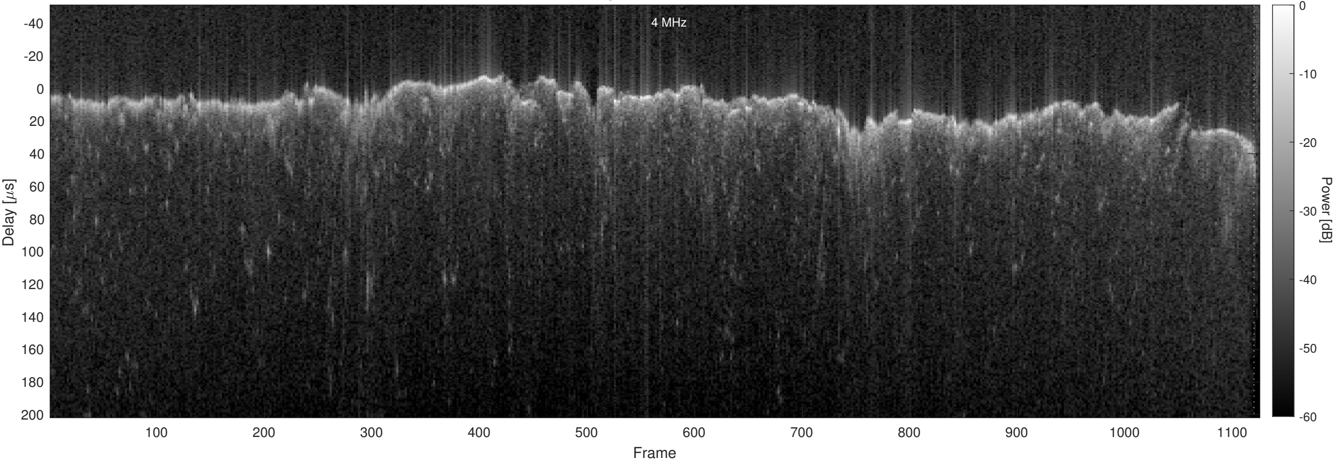
Orbit 22875, Chapman, No Window, Channel 2
