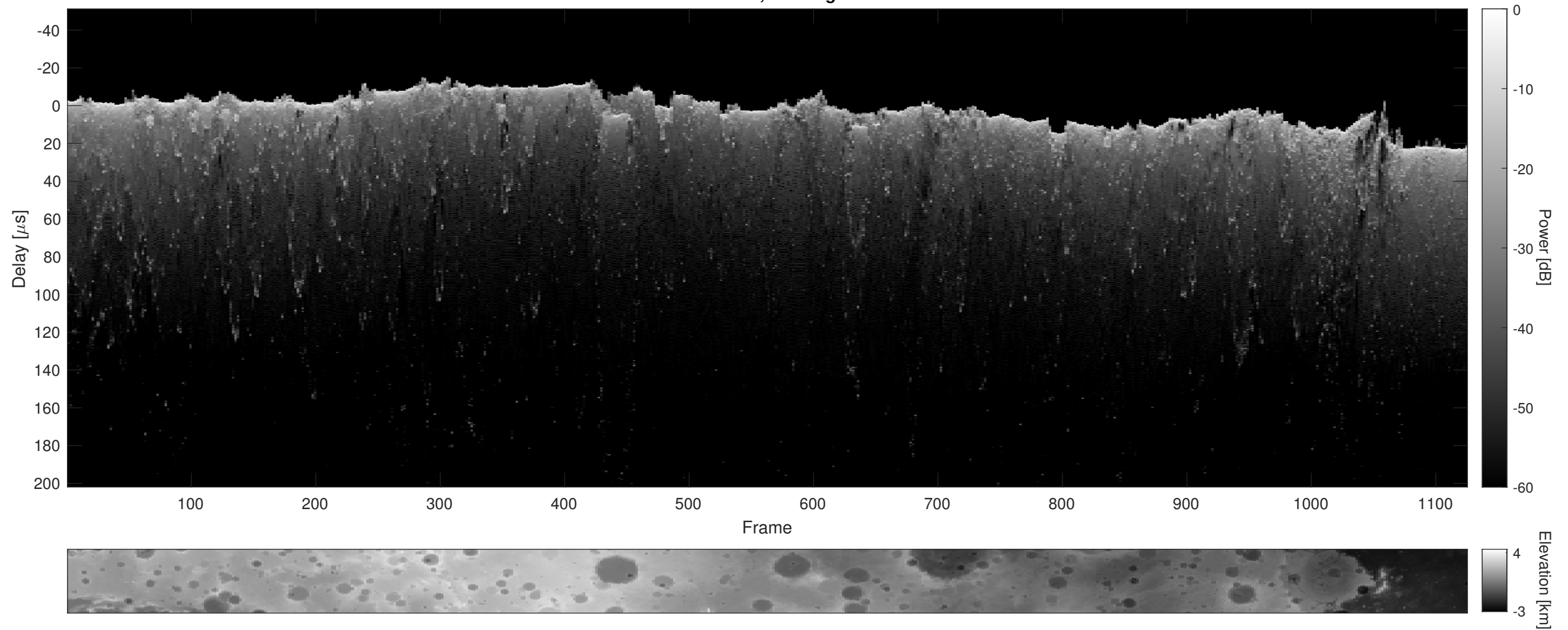
Orbit 22875, Cluttergram
