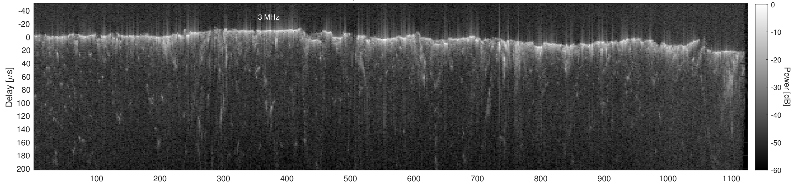
Orbit 22875, Cluttergram
