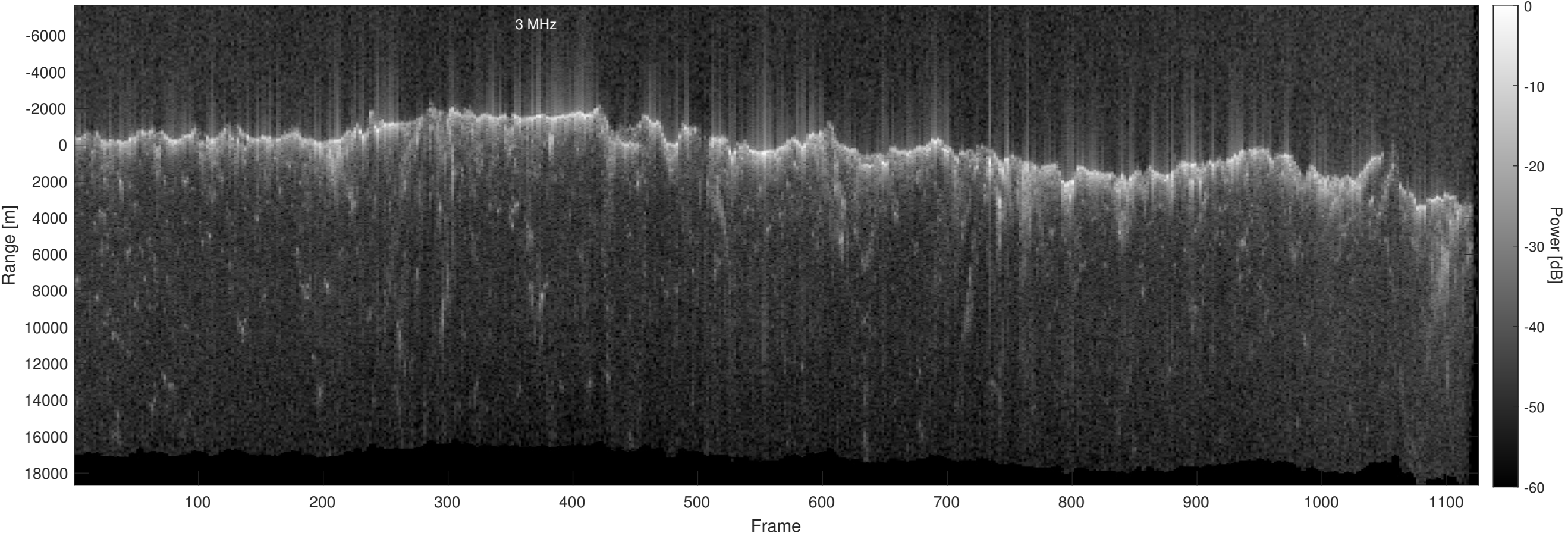
Orbit 22875, Optimized, No Window, Depth-Corrected, Channel 2
