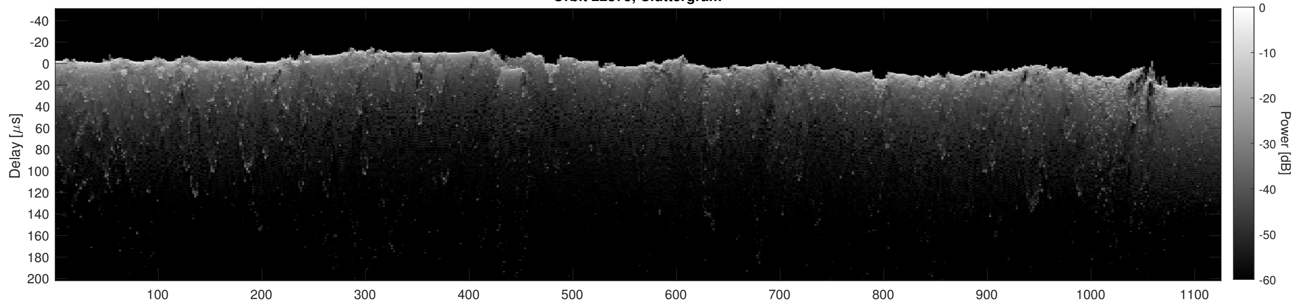
Orbit 22875, Cluttergram
