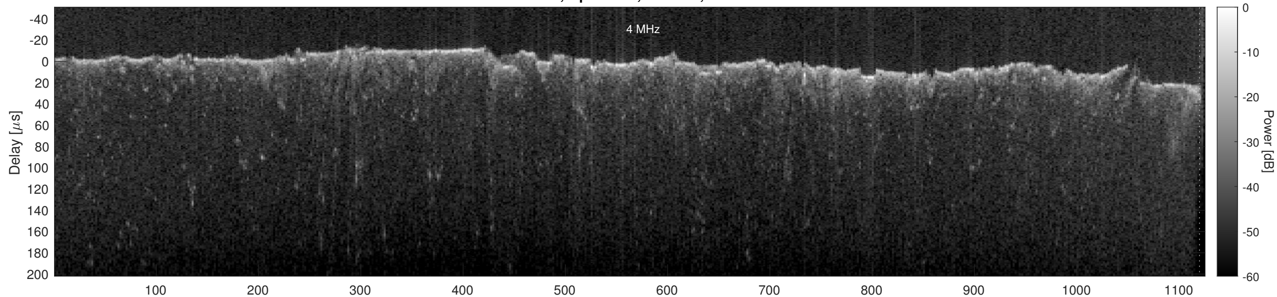
Orbit 22875, Optimized, Window, Channel 2
