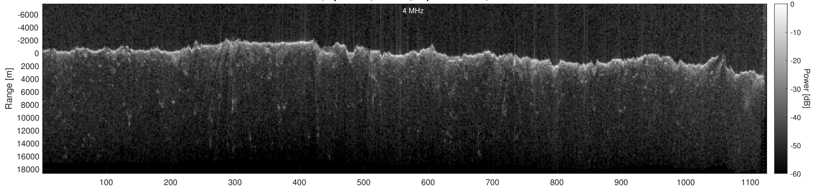
Orbit 22875, Optimized, Window, Depth-Corrected, Channel 2
