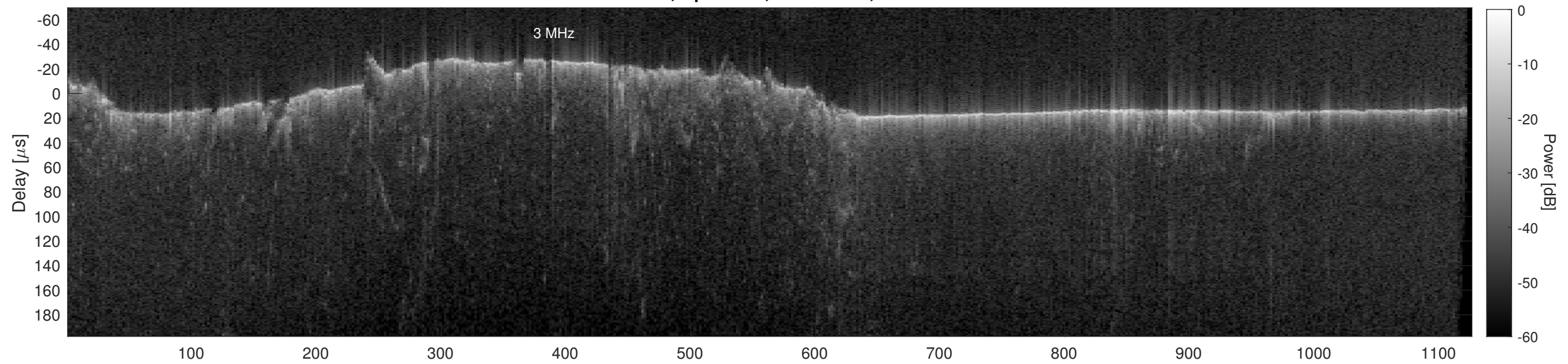
Orbit 22878, Cluttergram
