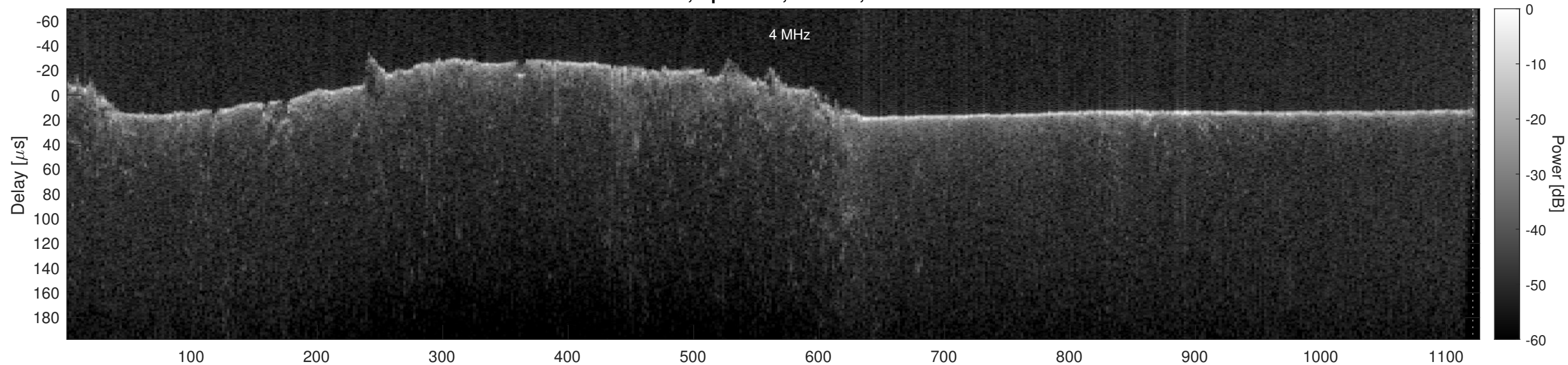
Orbit 22878, Optimized, Window, Channel 2
