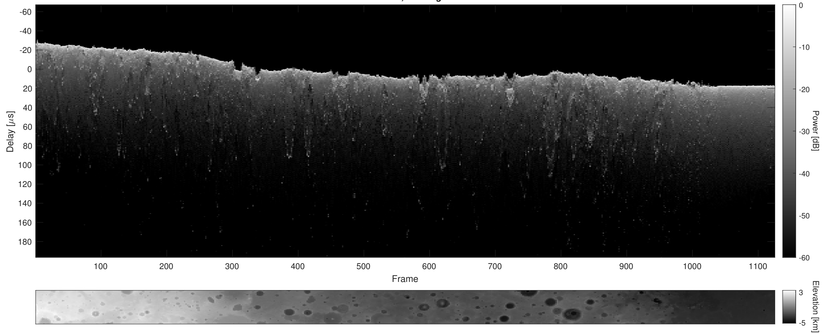
Orbit 22879, Cluttergram
