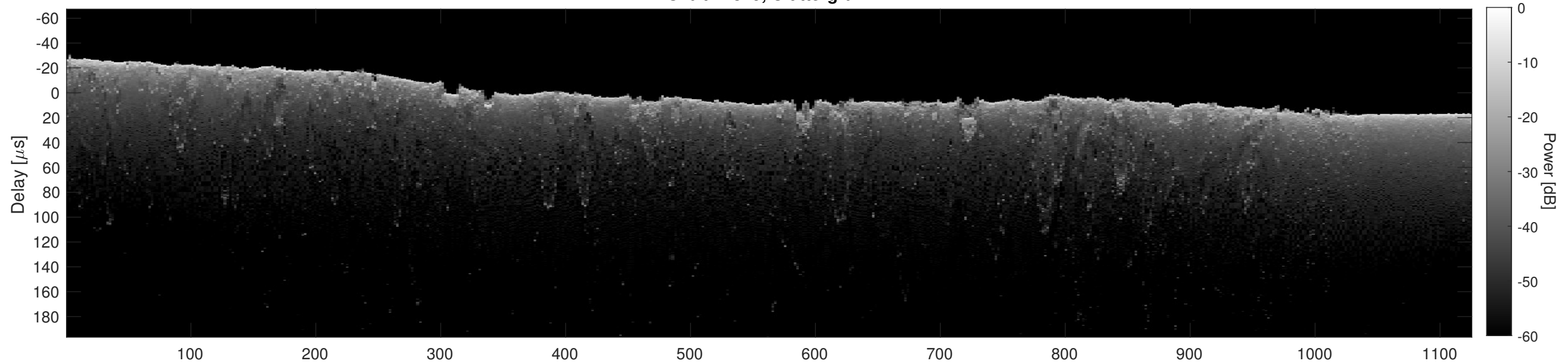
Orbit 22879, Cluttergram
