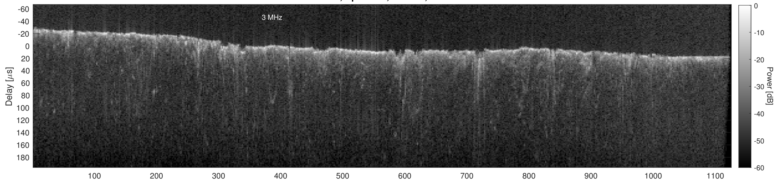
Orbit 22879, Cluttergram
