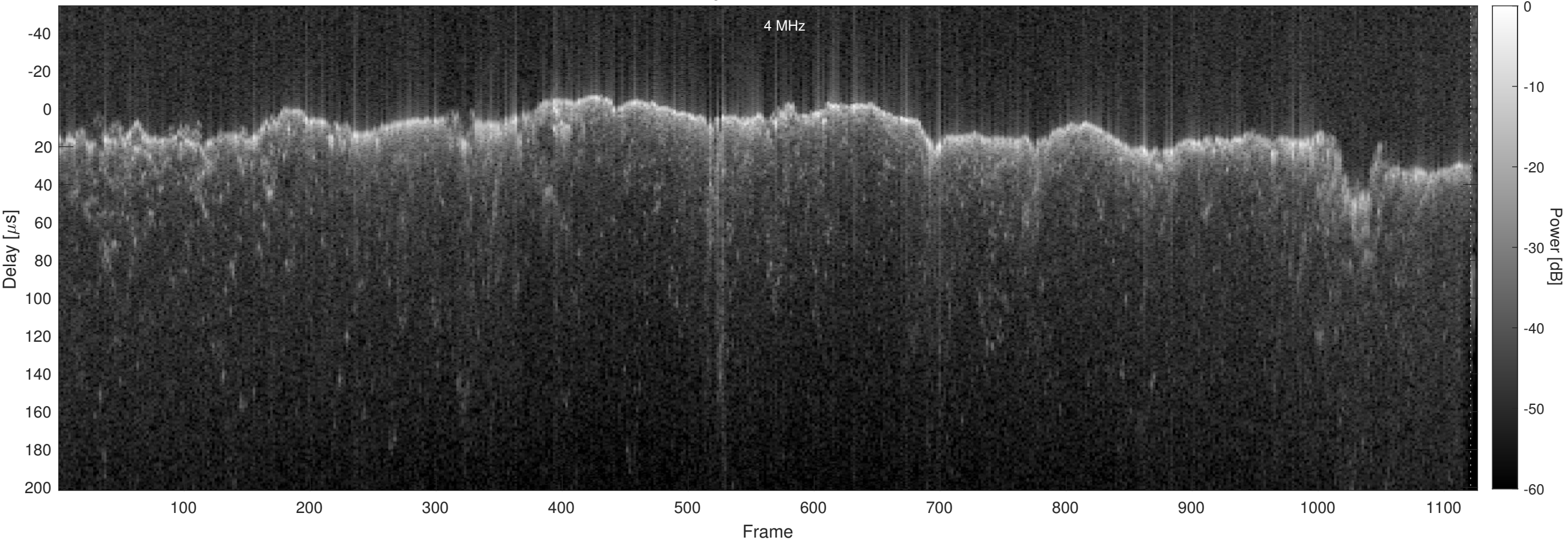
Orbit 22882, Chapman, No Window, Channel 2
