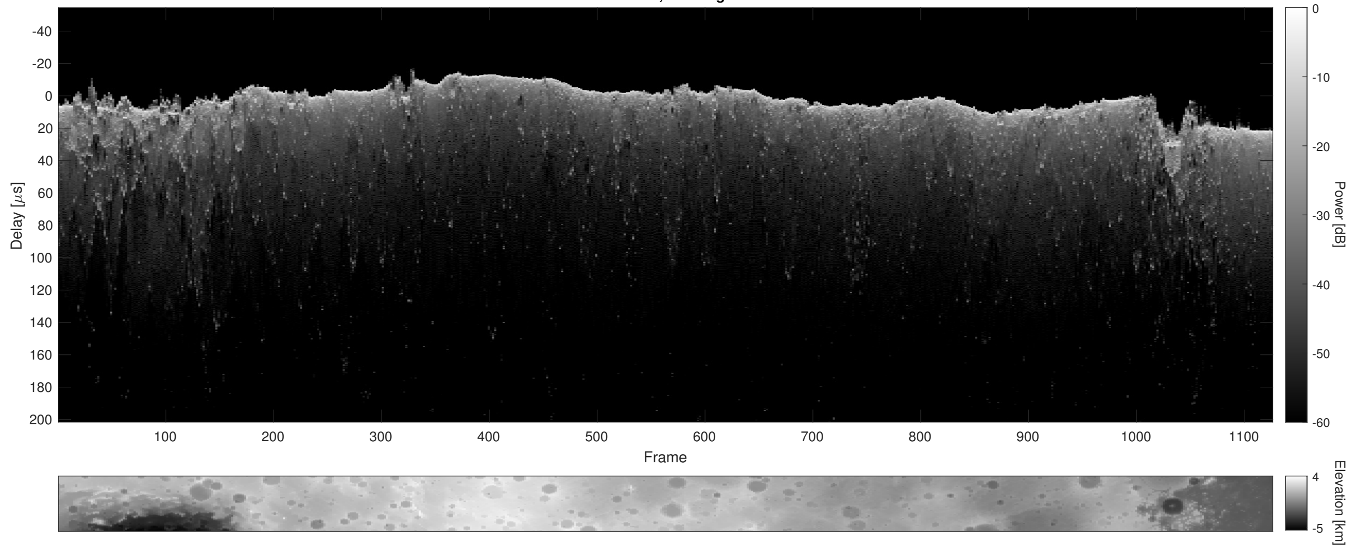
Orbit 22882, Cluttergram
