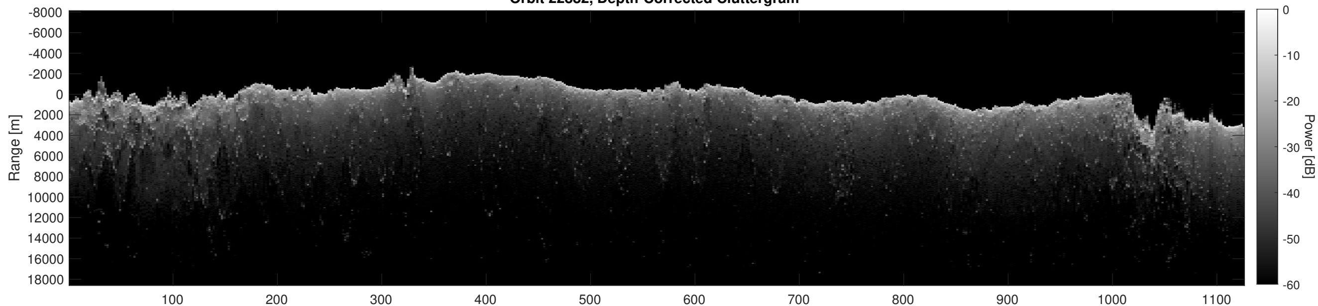
Orbit 22882, Depth-Corrected Cluttergram
