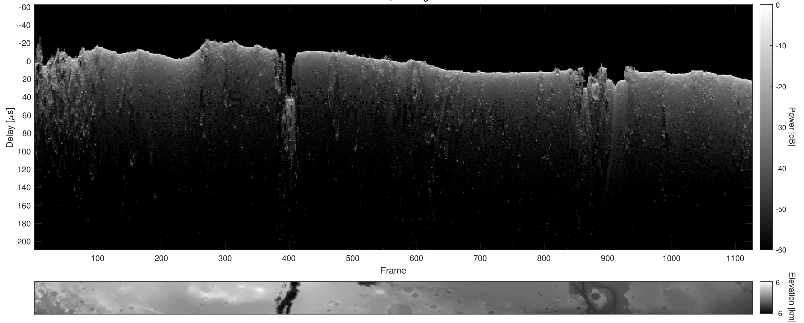
Orbit 22883, Cluttergram
