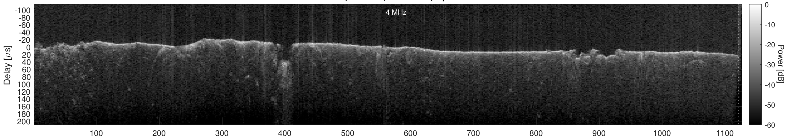
Orbit 22883, Cluttergram
