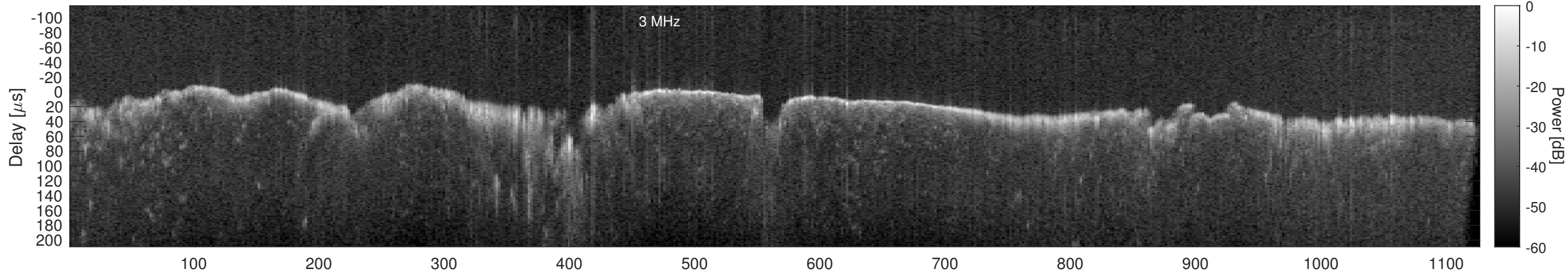
Orbit 22883, Window, Channel 2, Chapman
