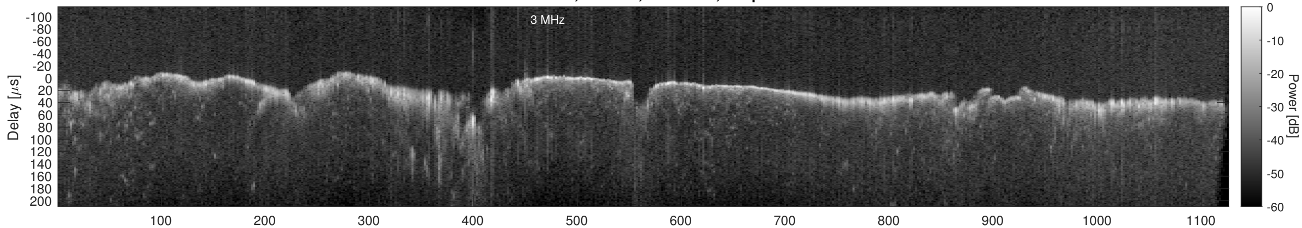
Orbit 22883, Window, Channel 2, Optimized
