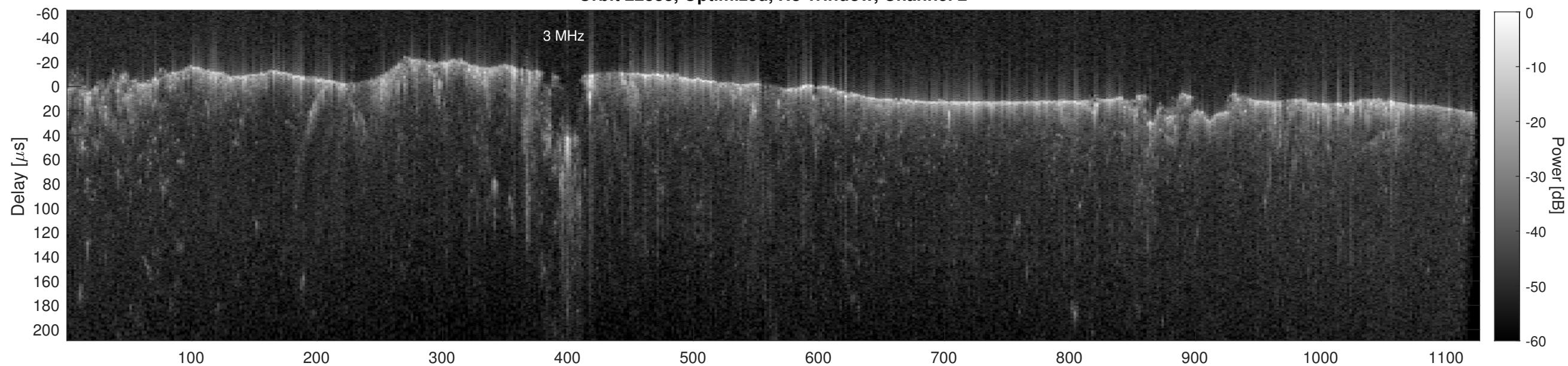
Orbit 22883, Cluttergram
