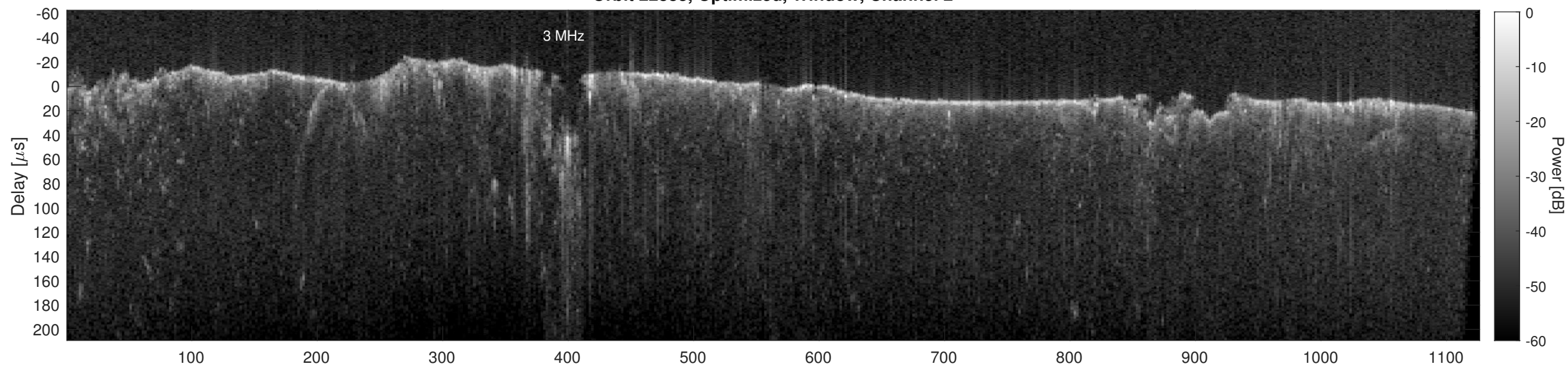
Orbit 22883, Cluttergram
