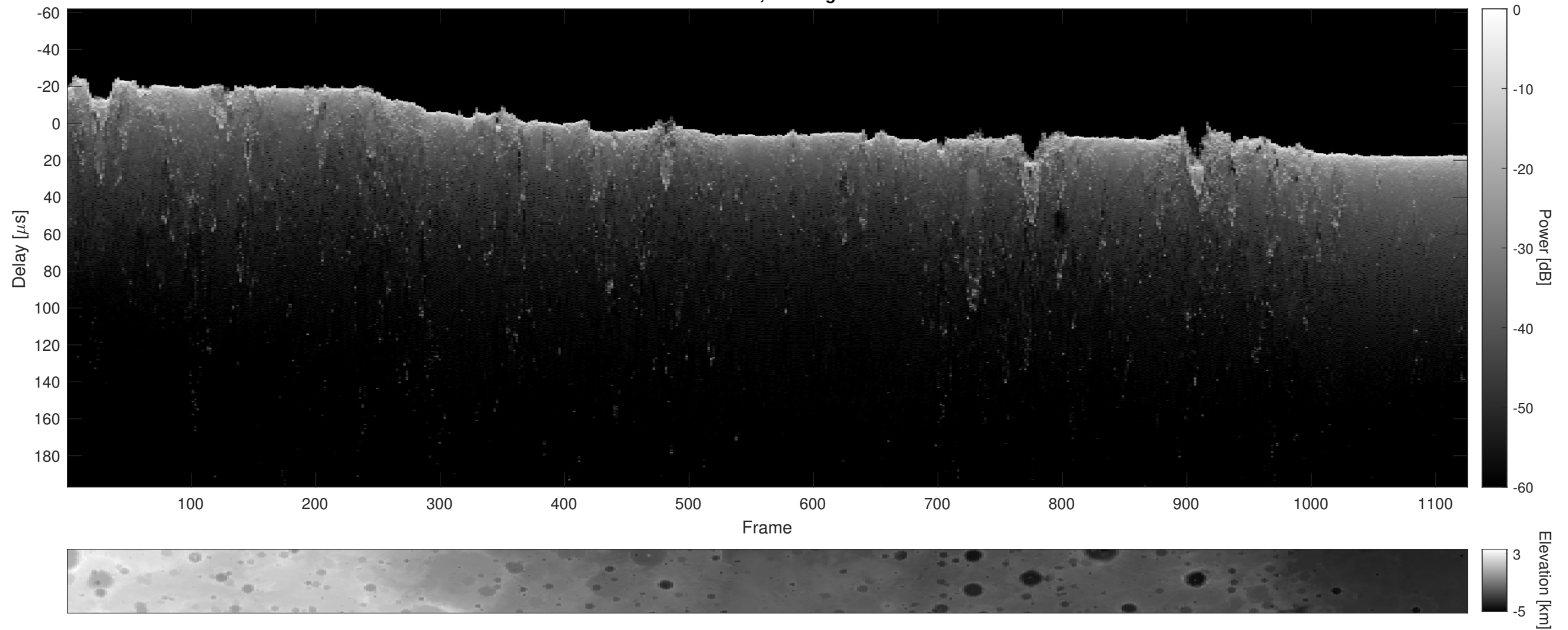
Orbit 22886, Cluttergram
