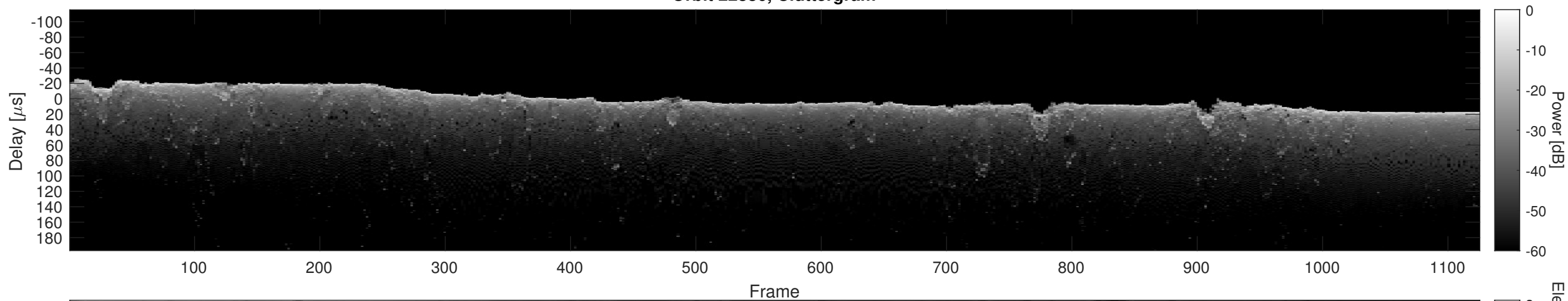
Orbit 22886, Cluttergram
