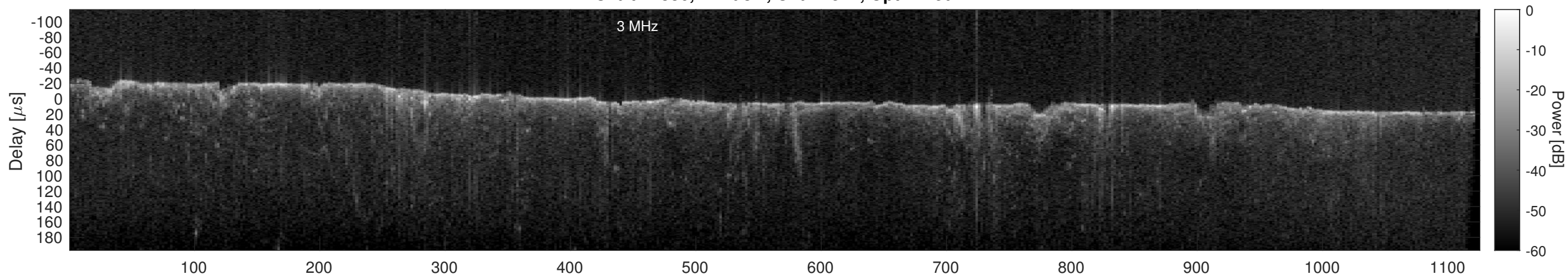
Orbit 22886, Cluttergram
