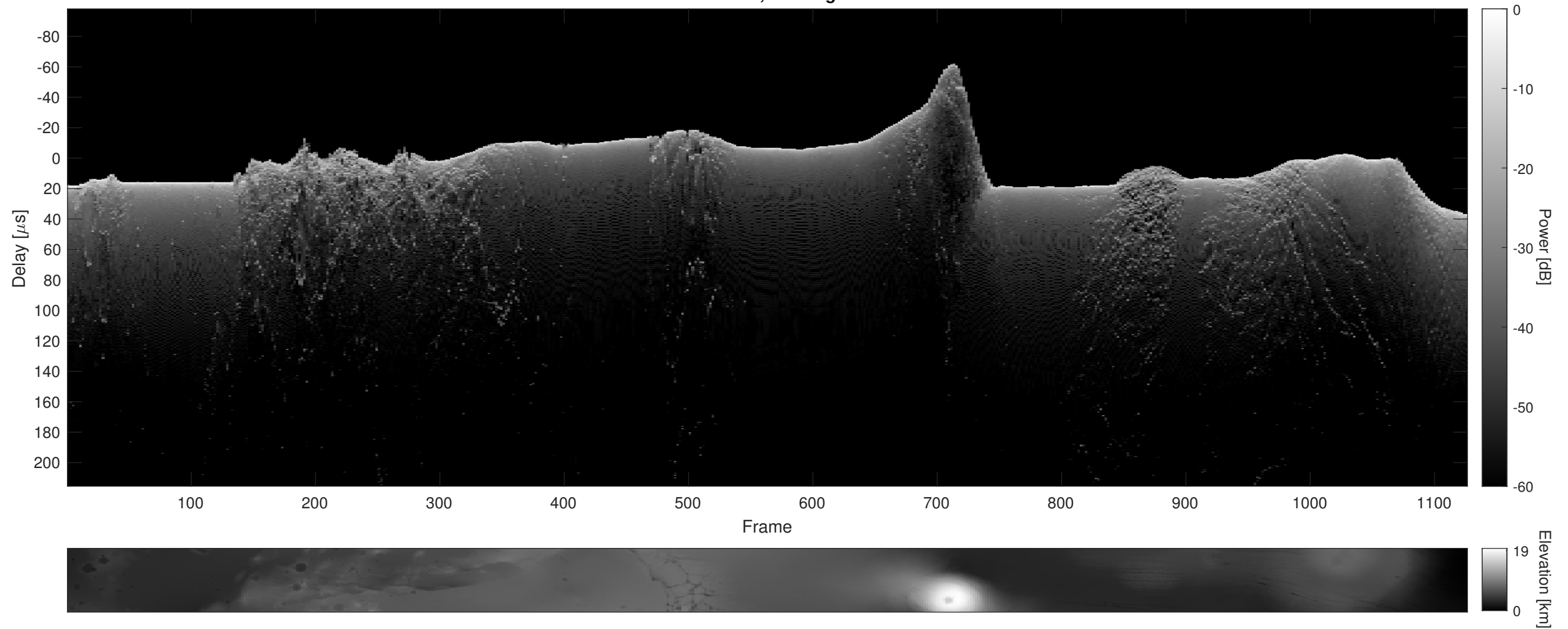
Orbit 22887, Cluttergram
