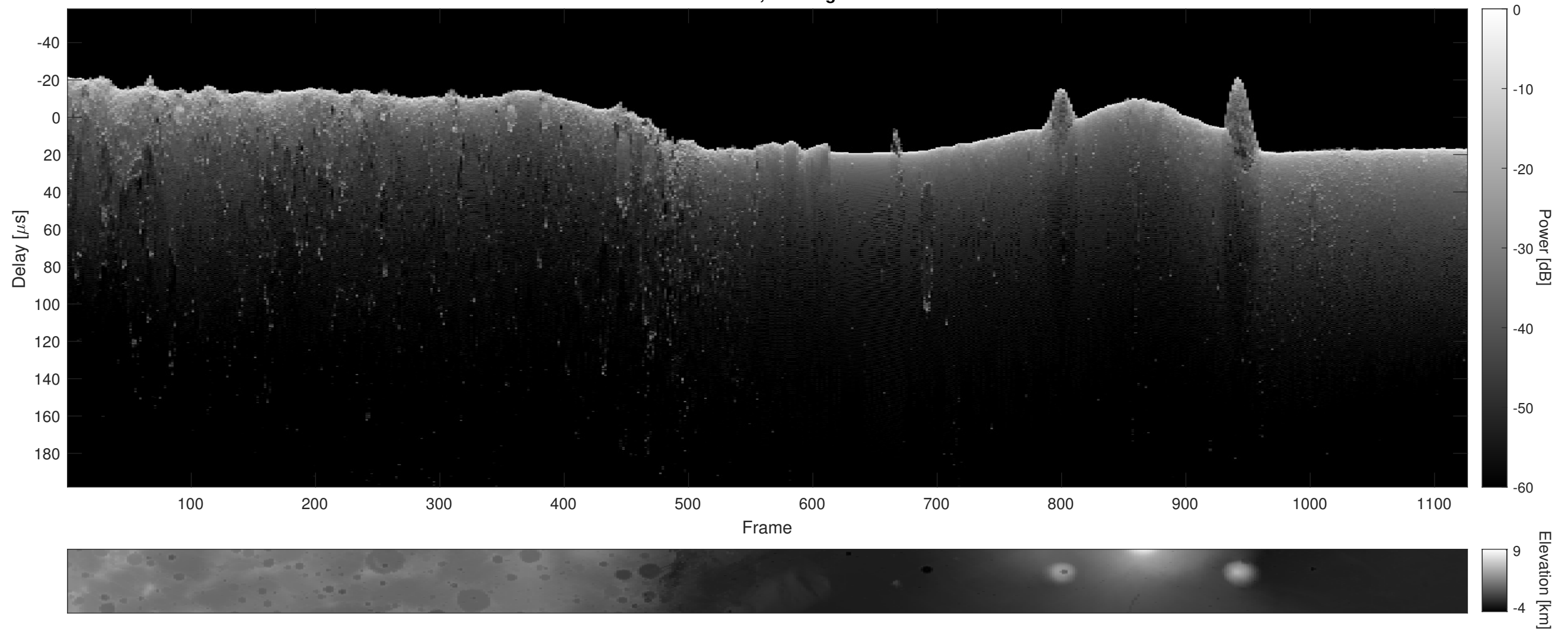
Orbit 22888, Cluttergram
