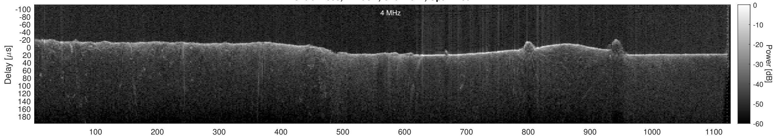
Orbit 22888, Cluttergram
