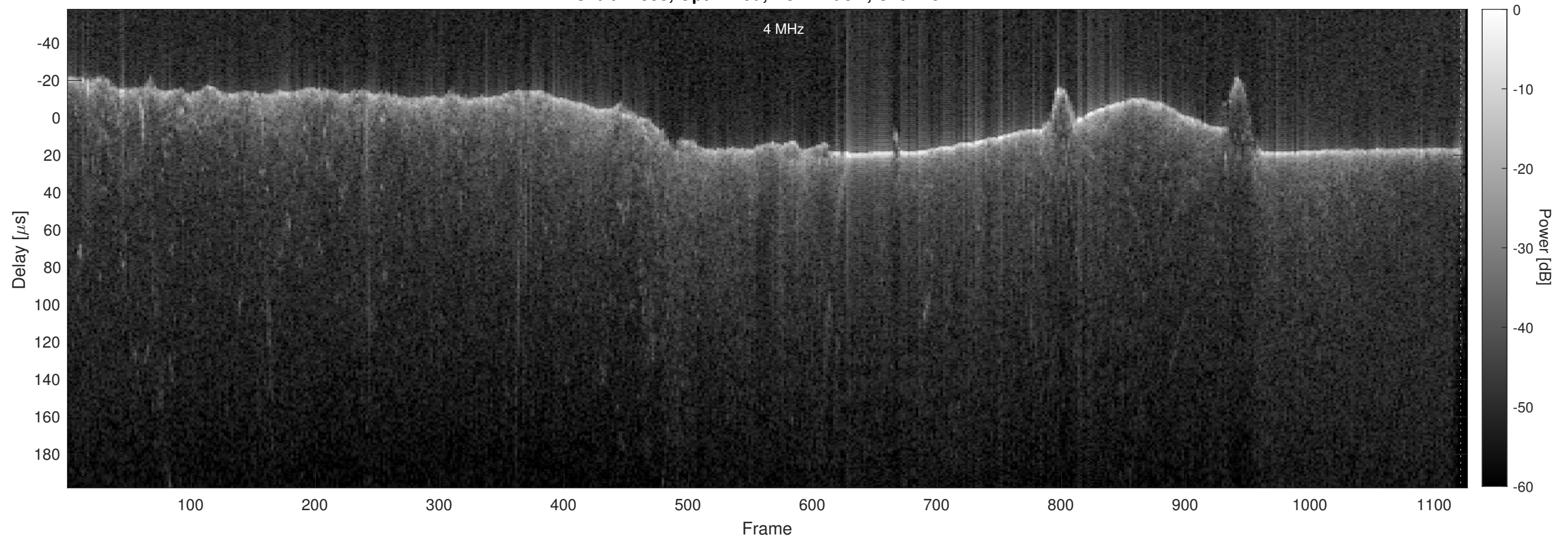
Orbit 22888, Optimized, No Window, Channel 2
