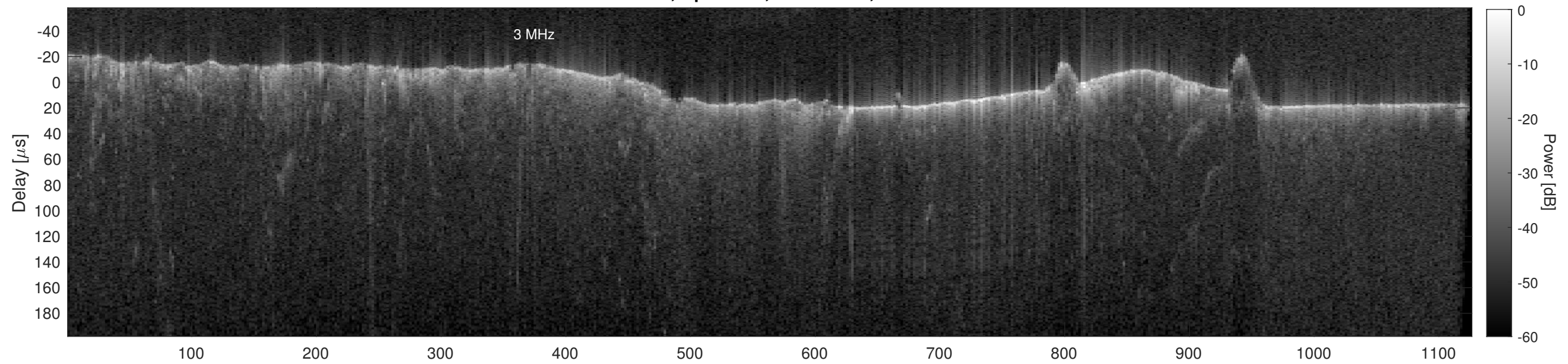
Orbit 22888, Cluttergram
