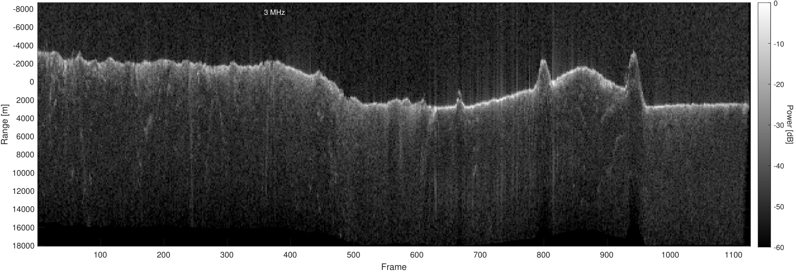
Orbit 22888, Optimized, Window, Depth-Corrected, Channel 2
