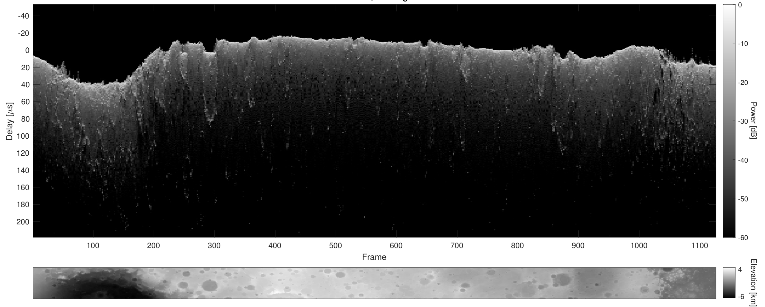
Orbit 22889, Cluttergram
