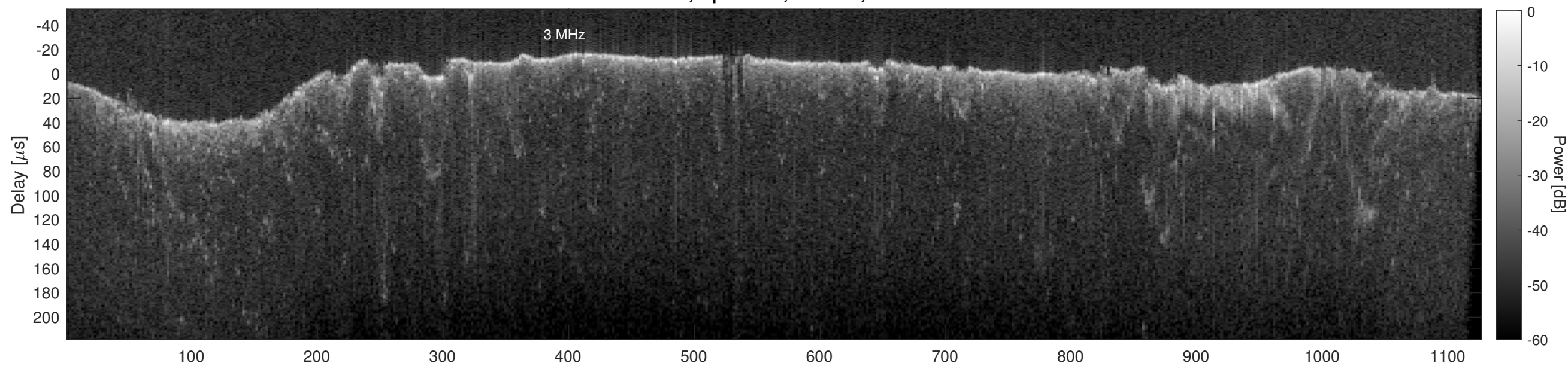
Orbit 22889, Cluttergram
