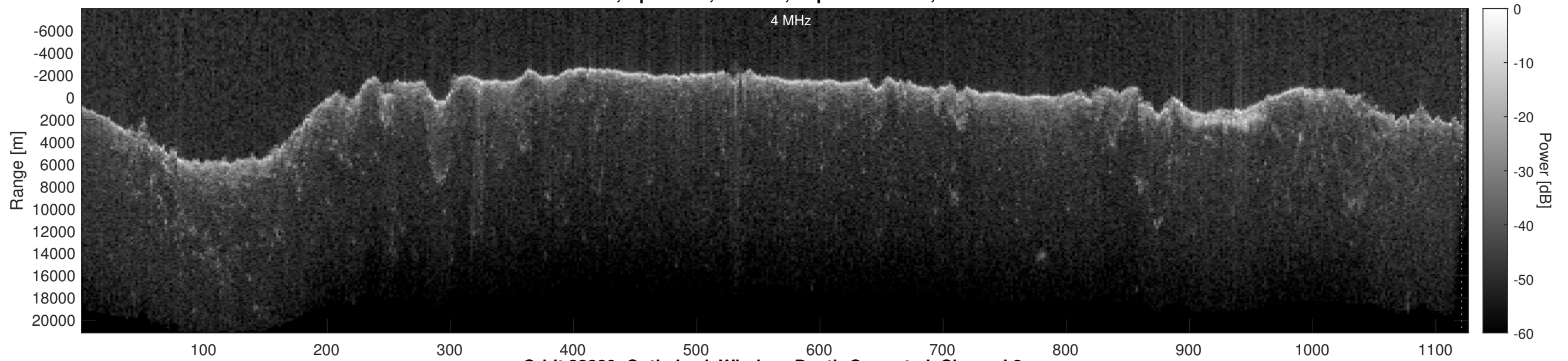
Orbit 22889, Optimized, Window, Depth-Corrected, Channel 2
