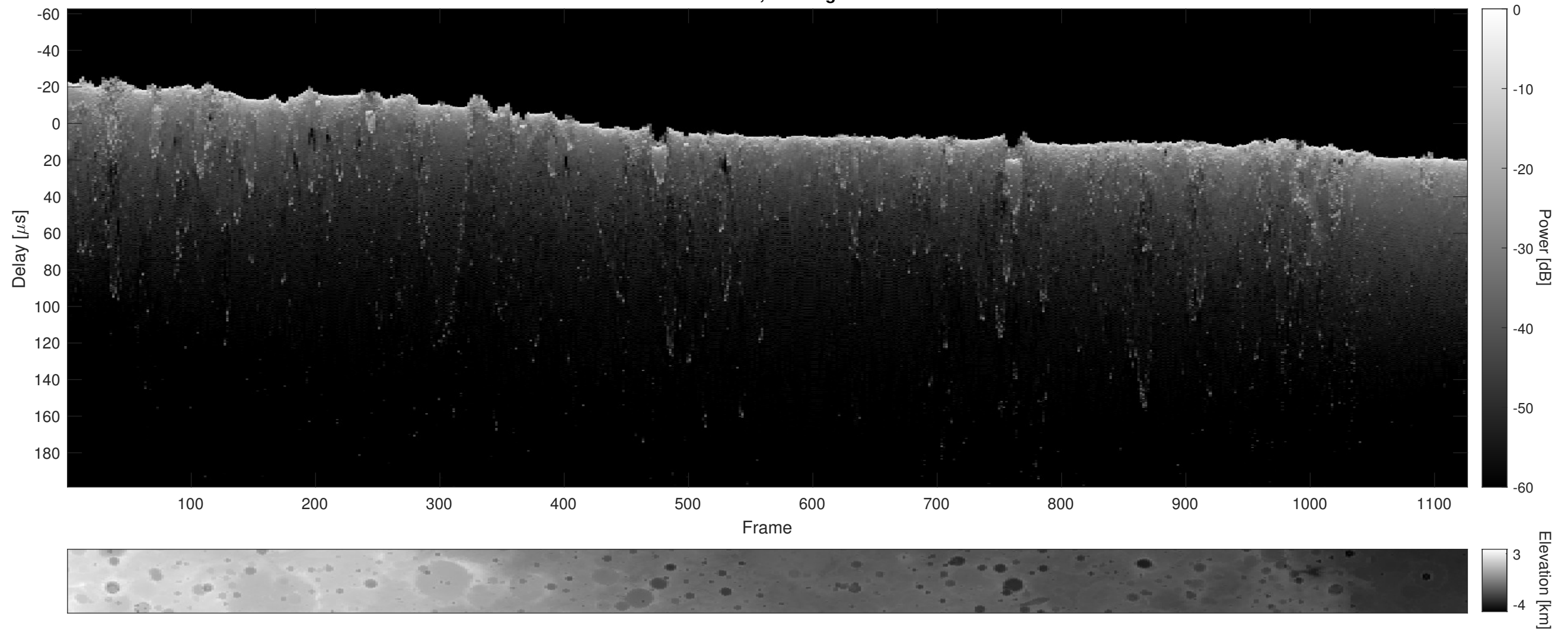
Orbit 22893, Cluttergram
