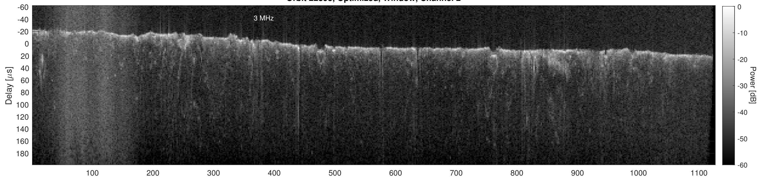
Orbit 22893, Cluttergram
