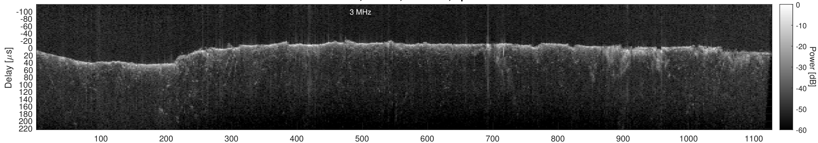
Orbit 22896, Cluttergram
