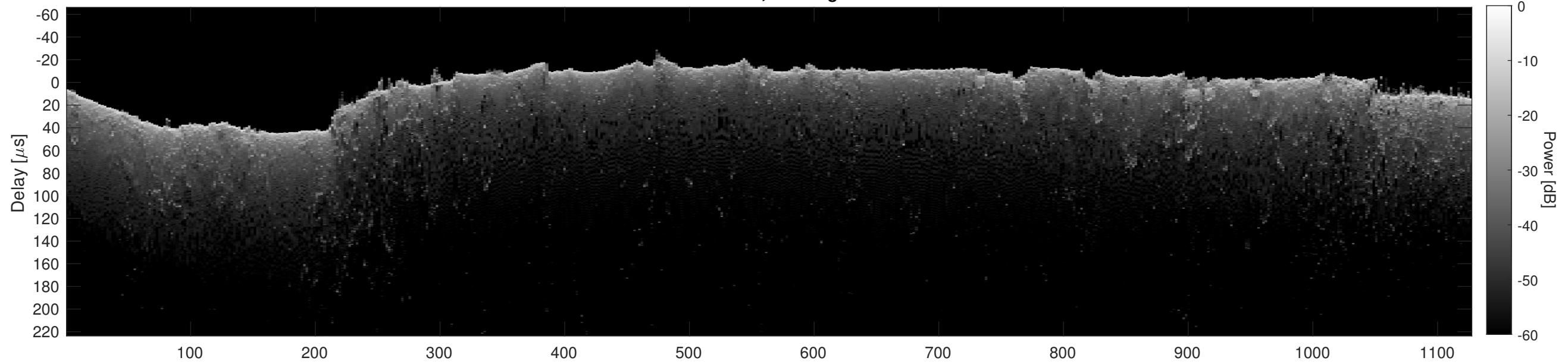
Orbit 22896, Cluttergram
