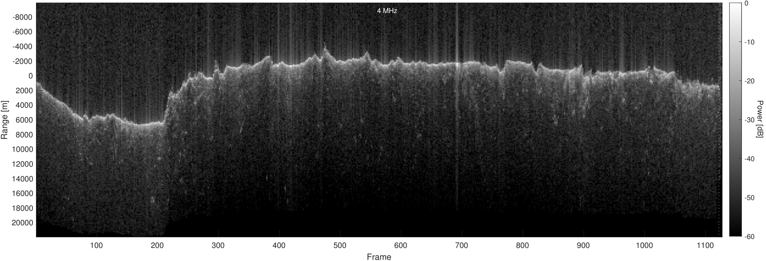
Orbit 22896, Optimized, No Window, Depth-Corrected, Channel 2
