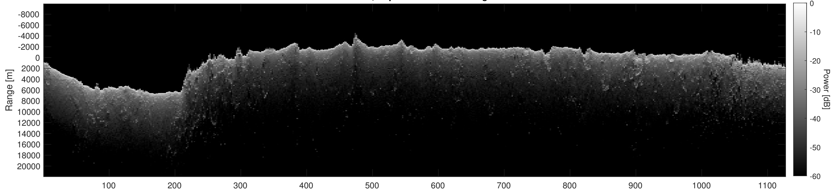
Orbit 22896, Depth-Corrected Cluttergram
