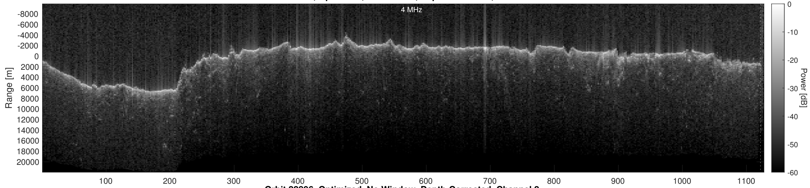
Orbit 22896, Optimized, No Window, Depth-Corrected, Channel 2
