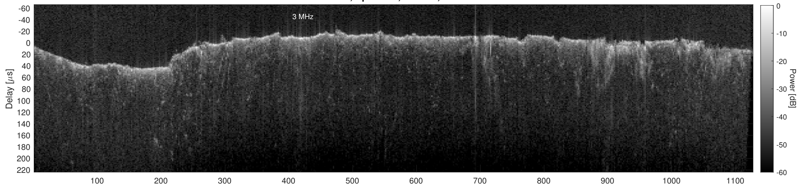
Orbit 22896, Cluttergram
