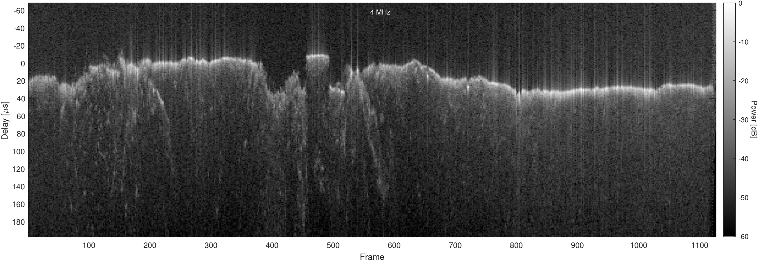
Orbit 22897, Chapman, No Window, Channel 2
