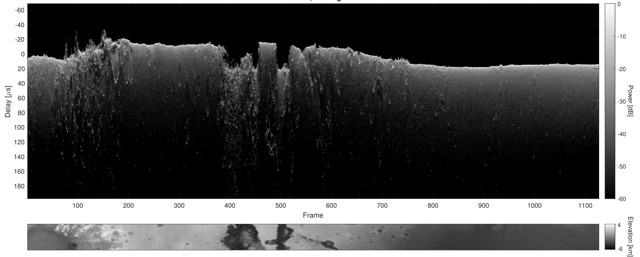
Orbit 22897, Cluttergram
