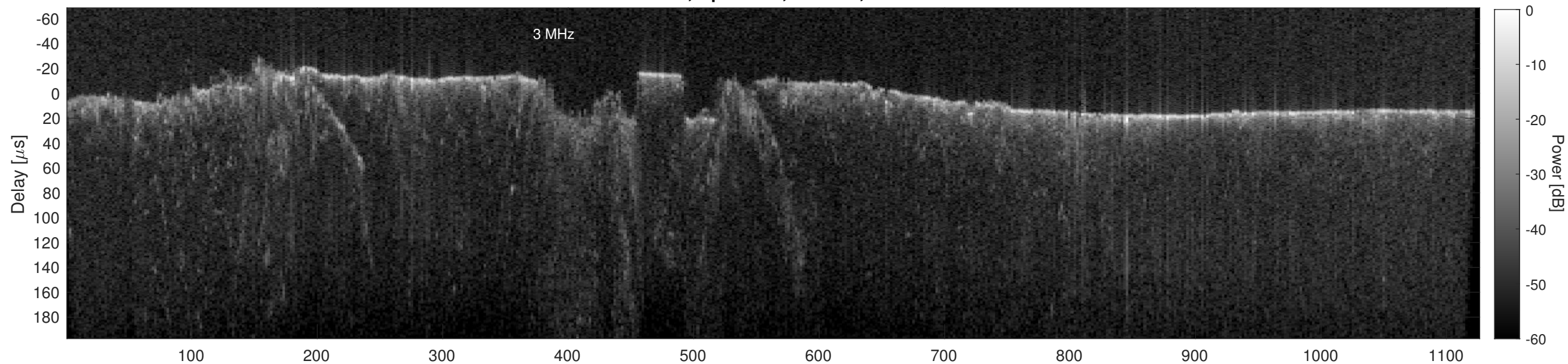
Orbit 22897, Cluttergram
