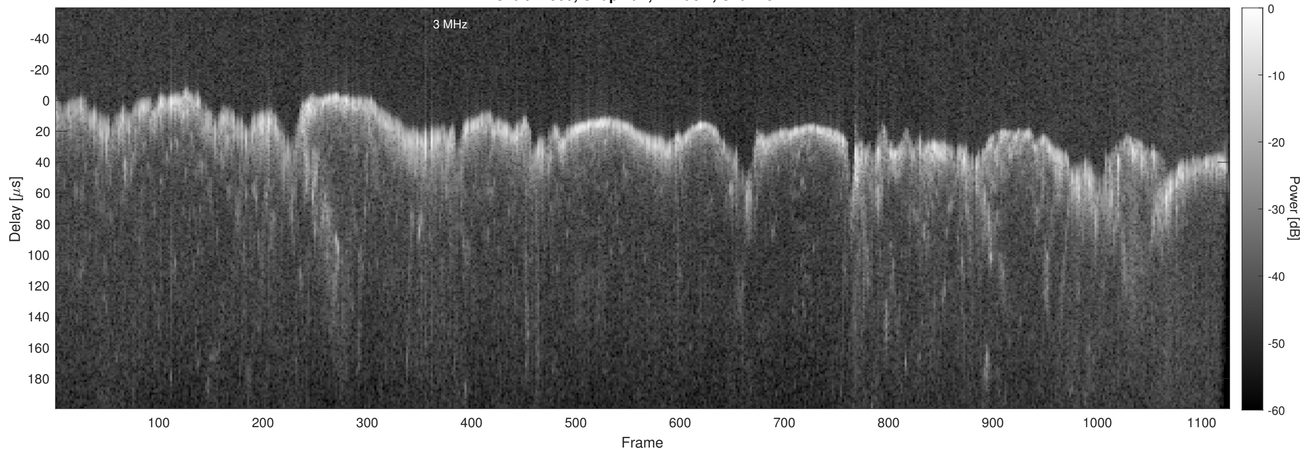
Orbit 22900, Chapman, Window, Channel 2
