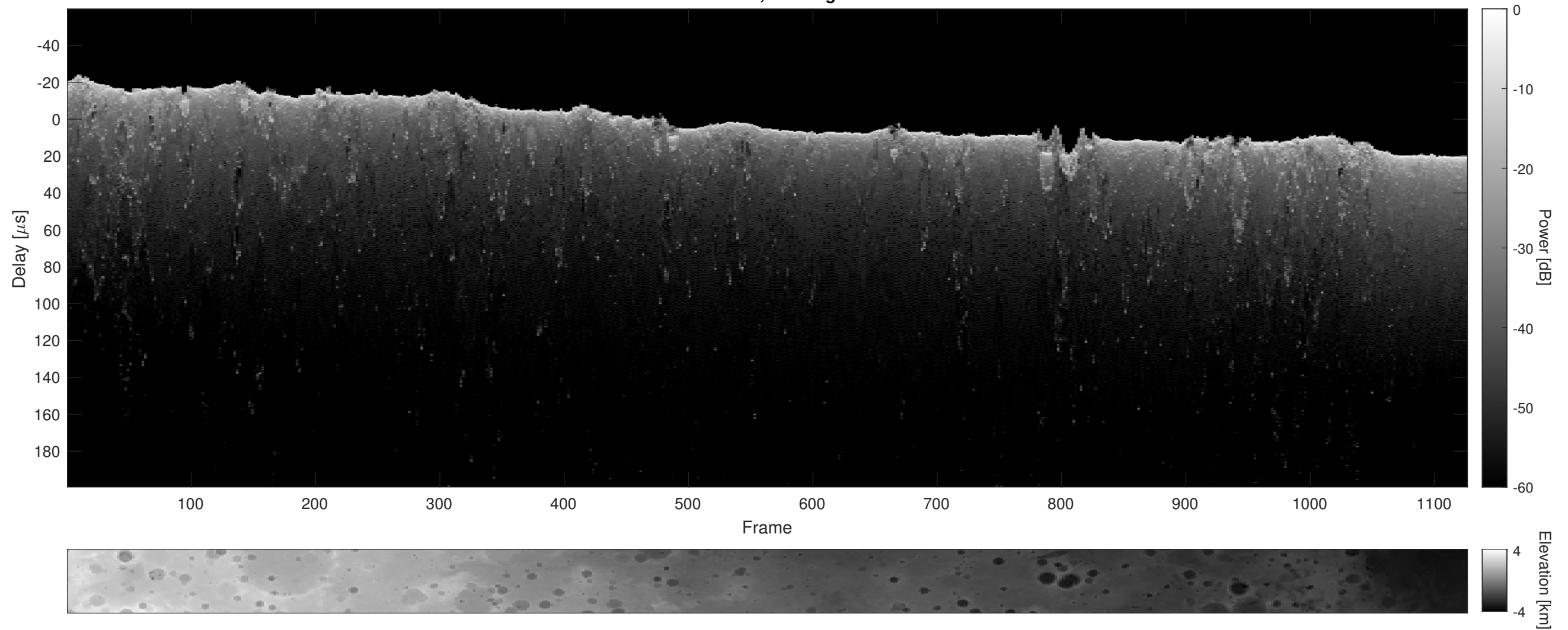
Orbit 22900, Cluttergram
