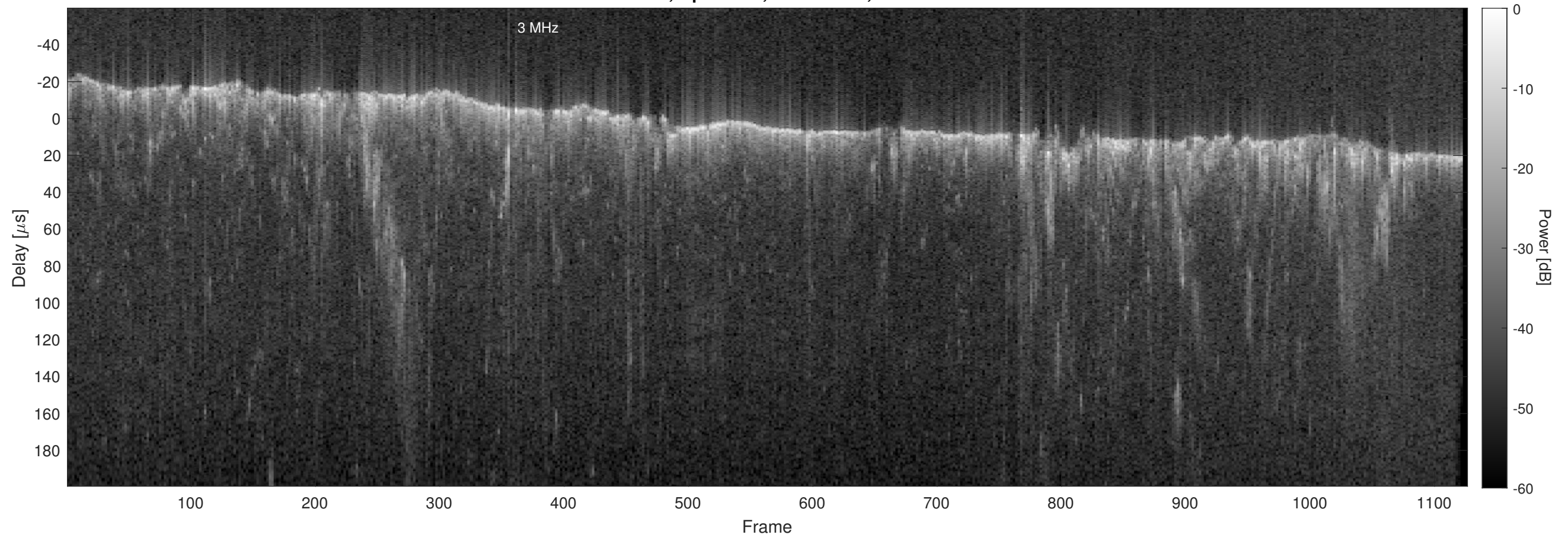
Orbit 22900, Optimized, No Window, Channel 2
