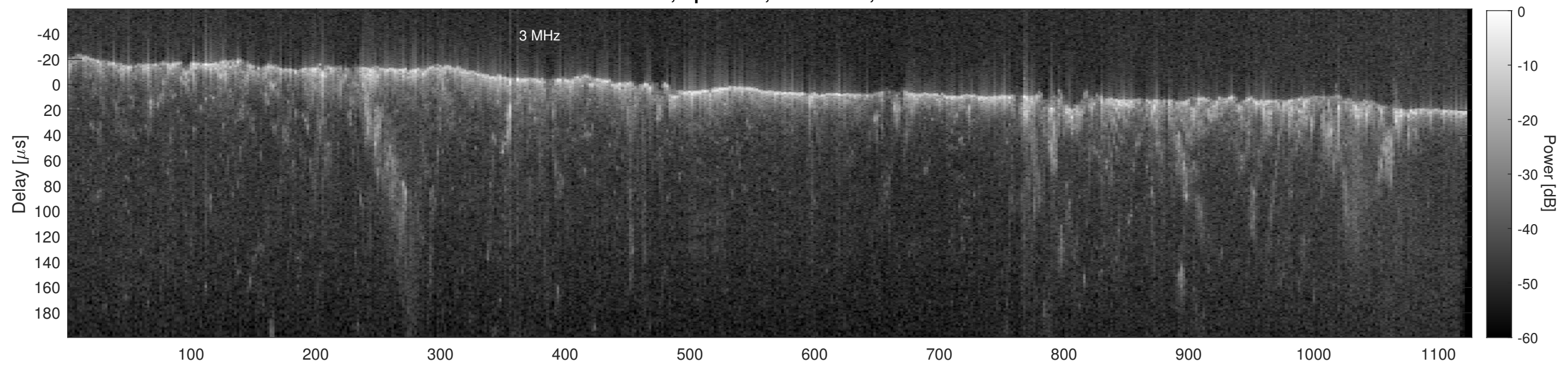
Orbit 22900, Cluttergram
