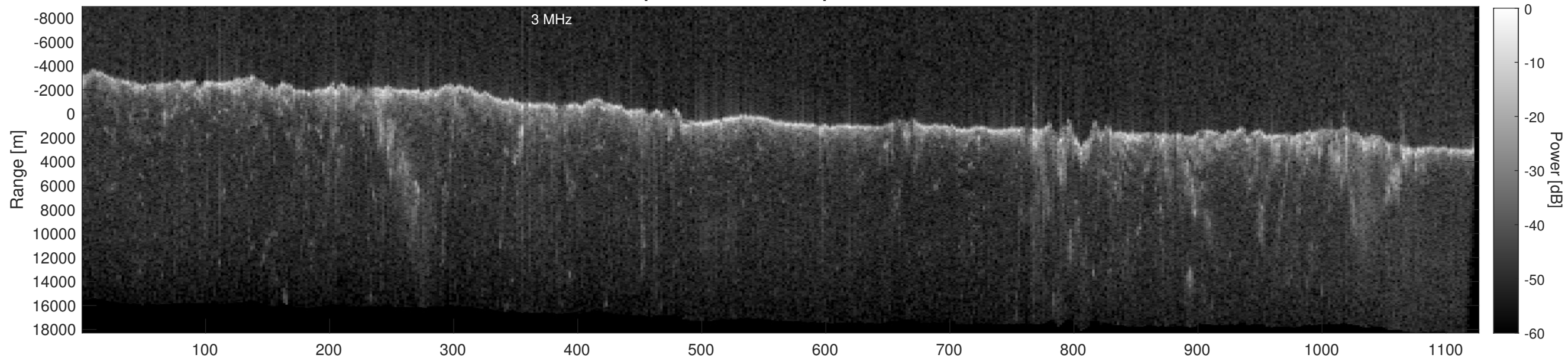
Orbit 22900, Depth-Corrected Cluttergram
