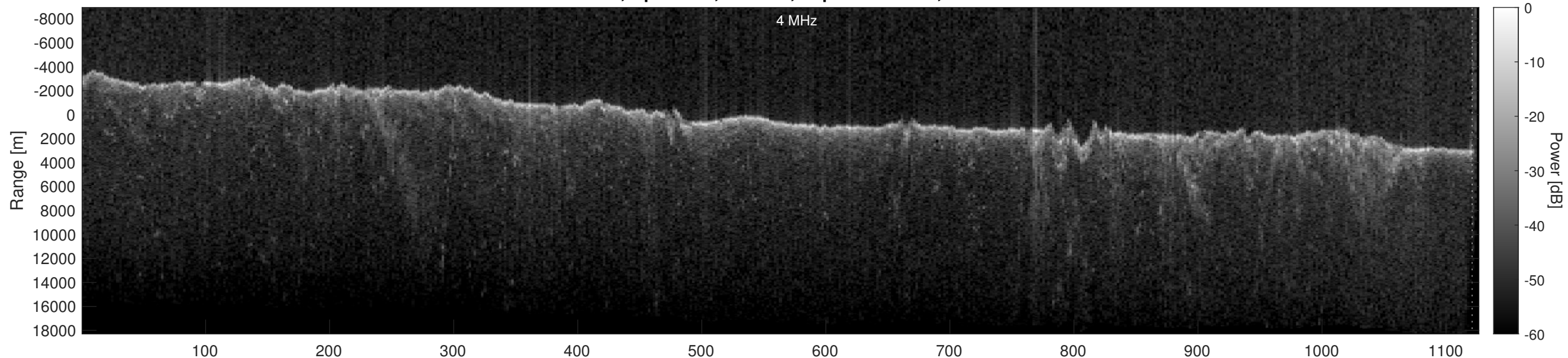
Orbit 22900, Optimized, Window, Depth-Corrected, Channel 2
